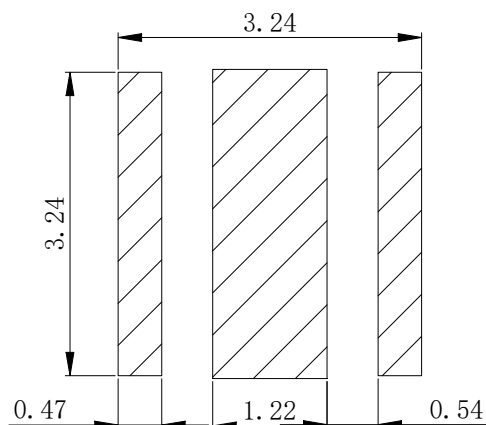
Recommended pad
