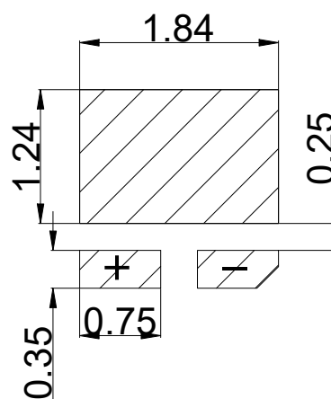
Recommended pad
