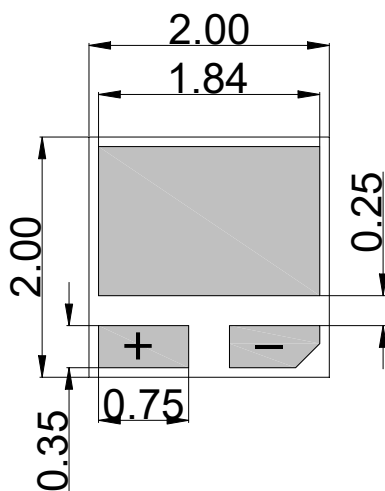
Perspective View
